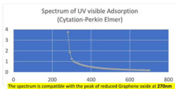
Figure 30. The spectroscopy UV analysis showed an adsorption due to the presence of reduced graphene oxide or graphene hydroxide, which is confirmed by observation under ultraviolet visible microscopy.
