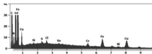
Figure 41 shows the quantified nano particulates in the Astrazeneca vaccine with an x-ray microprobe of an Energy Dispersive System that
