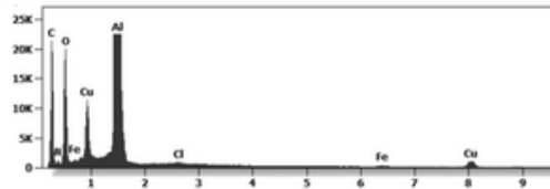
Figure 52 reveals Embedded Cytotoxic Nano Particulates. Figures 53 and 54 revealed the chemical nature of the observed micro and nano particulates. Many foreign bodies were identified with a spherical morphology with some bubble-shaped cavities.
