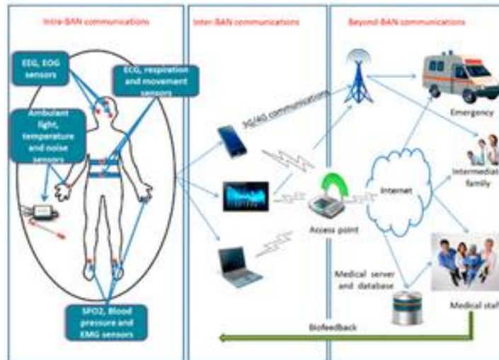
Figure 66. The General Architecture of Wireless Body Area Networks (WBANs)-based TRANS-HUMAN System. 148
